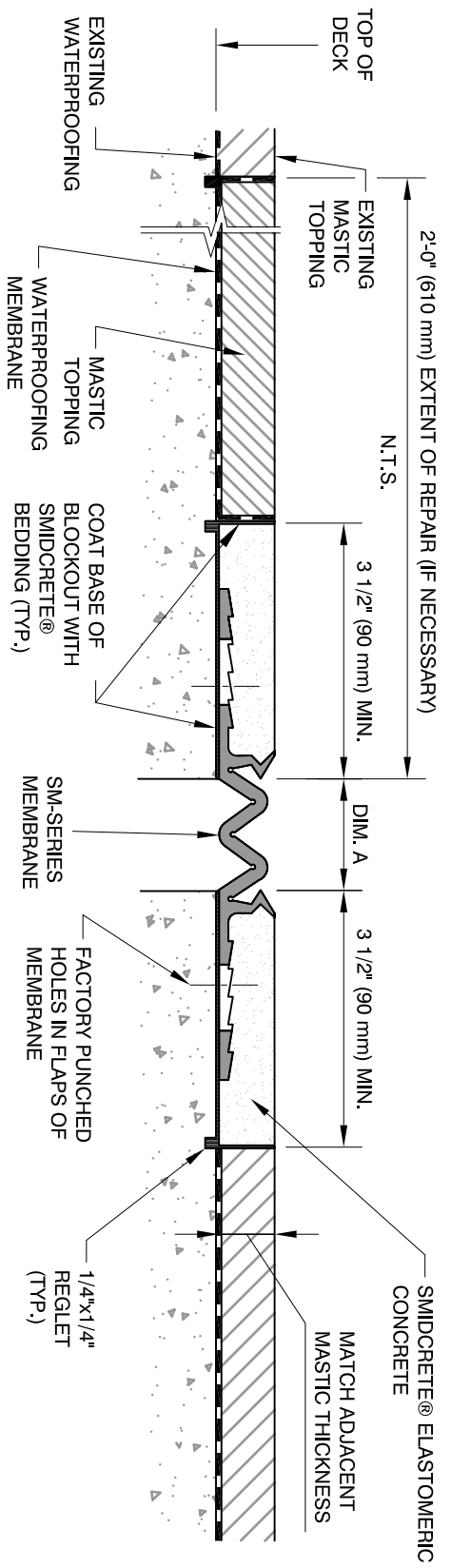
SLAB TO SLAB DETAIL
